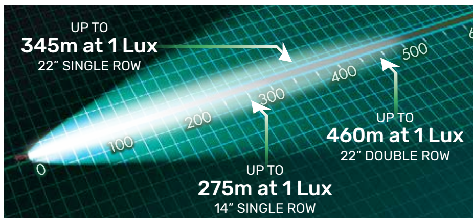
EXPLORA L.E.D LIGHT BAR BEAM PATTERNS
